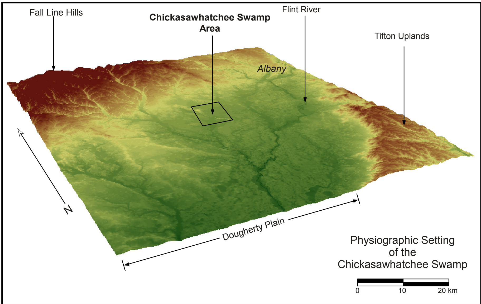
Figure 3: Digital Elevation Model with 10x Z factor exaggeration to show landscape features
